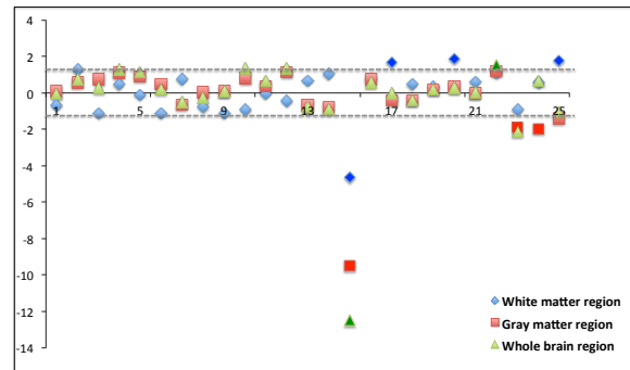
Fig. 4. Plot of all z-scores in the adult data. The dashed lines represent the cutoff the suspicious category.
